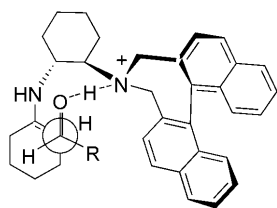
Figure 3. Proposed transition state model.
