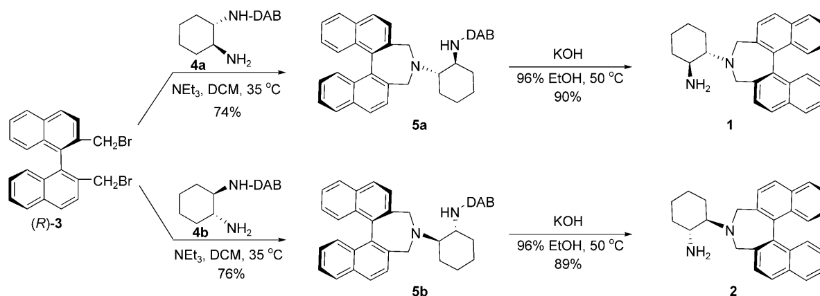
Scheme 1. Synthesis of bifunctional organocatalysts 1 and 2 .
