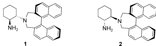
Figure 1. Designed bifunctional catalysts 1 and 2 .
