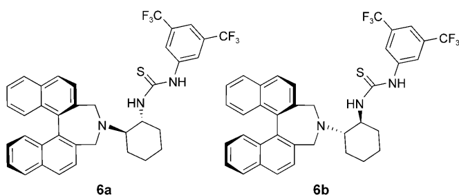
Figure 2. Bifunctional amine-thiourea organocatalysts 6a and 6b .
